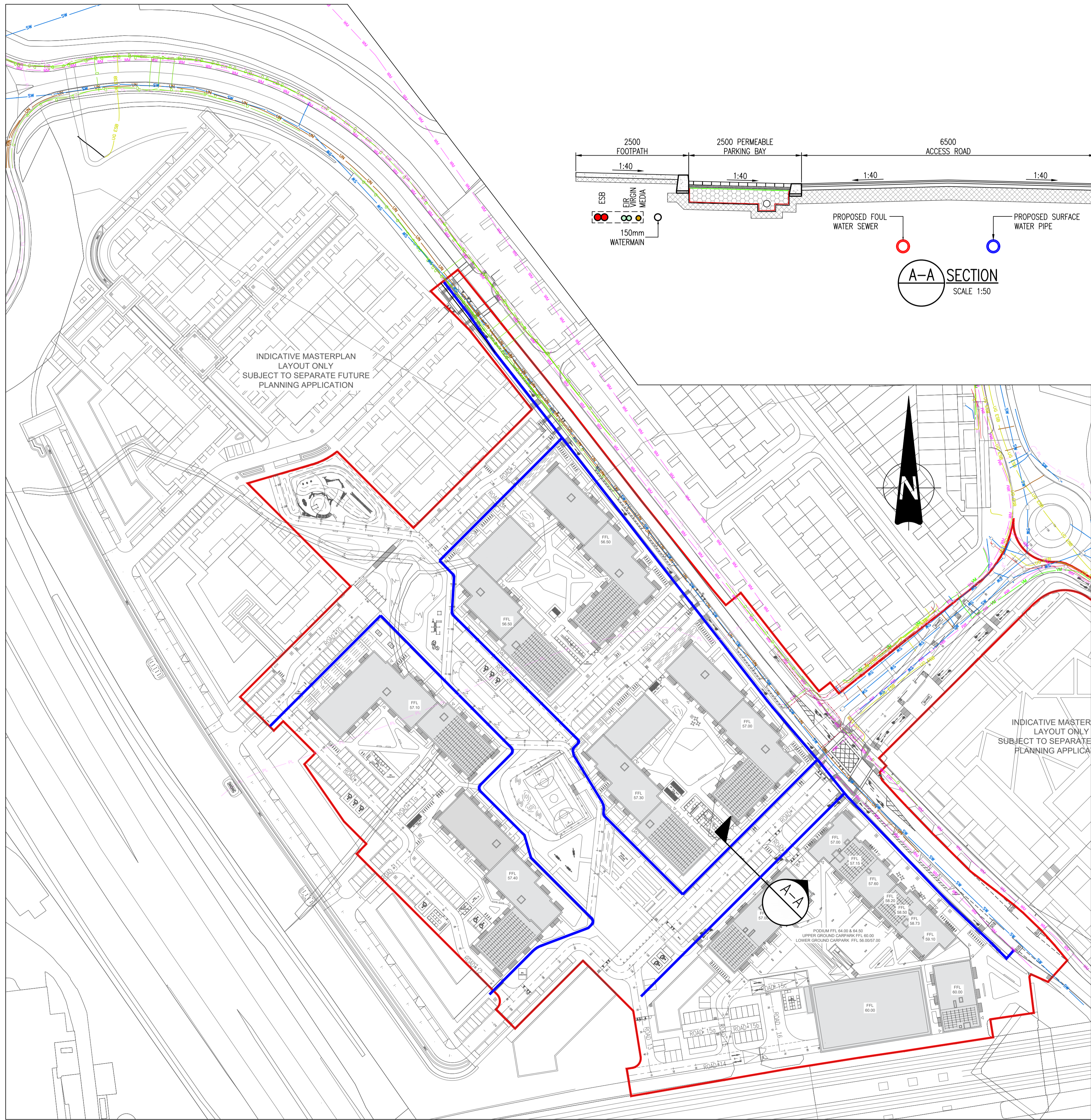
UTILITIES PLAN SCALE 1:1000
